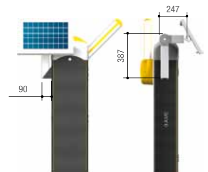
Applying the 001ZERO-E01 solar panel
